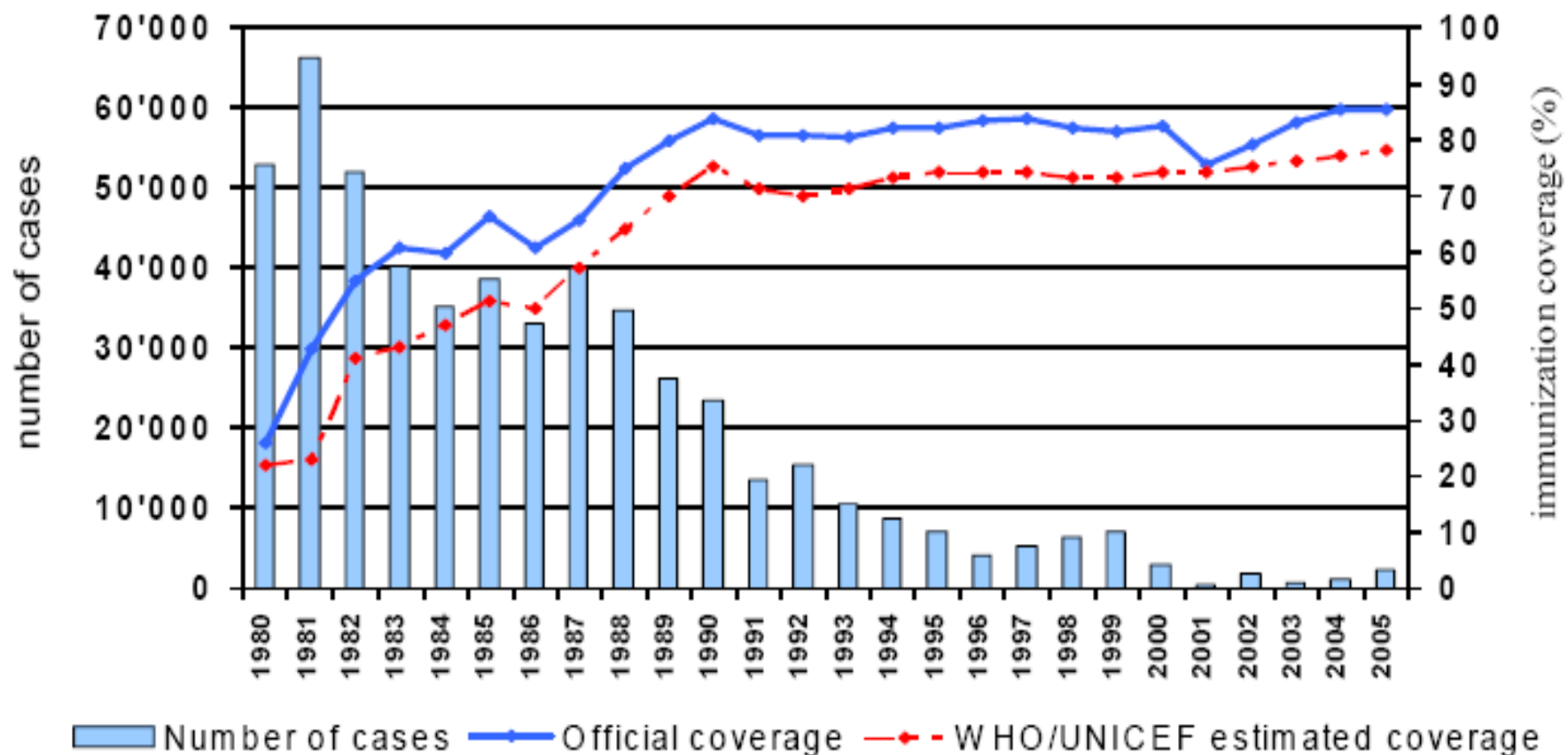
Poliomyelitis global annual reported incidence and Pol3 coverage, 1980-2005
